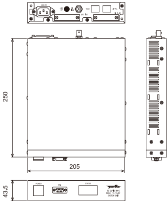
[ Dimensional Drawing ]
