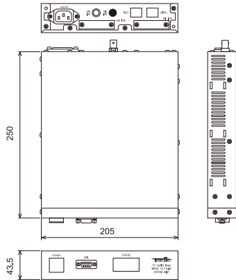
[ Dimensional Drawing ]
